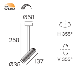
TL-2818 CANOPE
