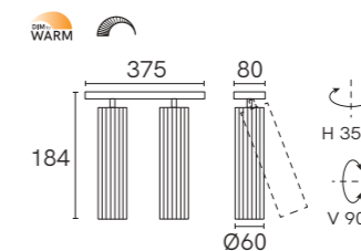
TL-2859.SOR
