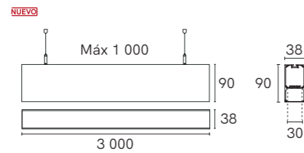
TL-4518.SUS KIT
