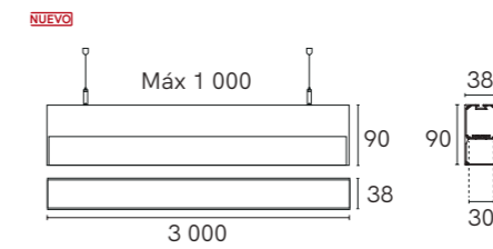
TL-4519.SUS KIT
