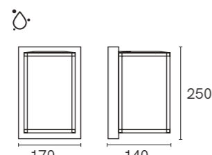
ML-4815.N30
