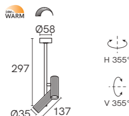
TL-2819 CANOPE
